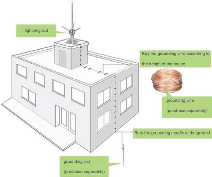
Early Streamer Emission Method LPS
