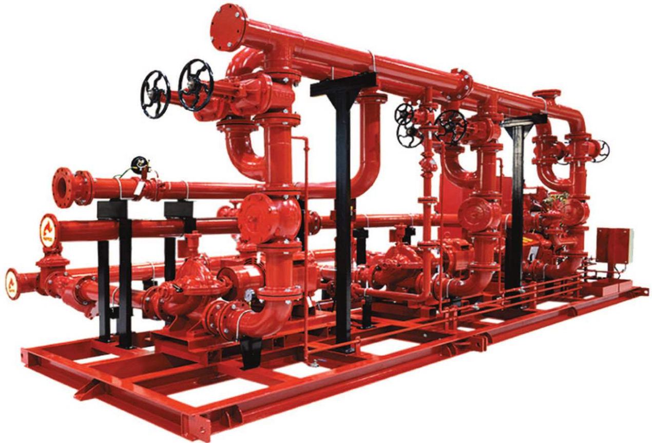
Fire Pump Set
