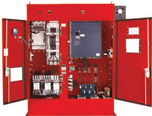
Fire Pump Controller
