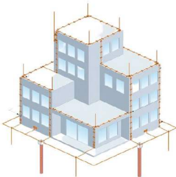
Conventional Method LPS
