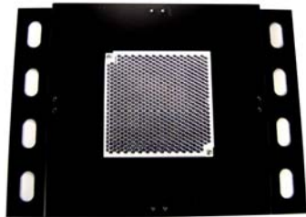
One Prism on 5000-006 Mounting Bracket
