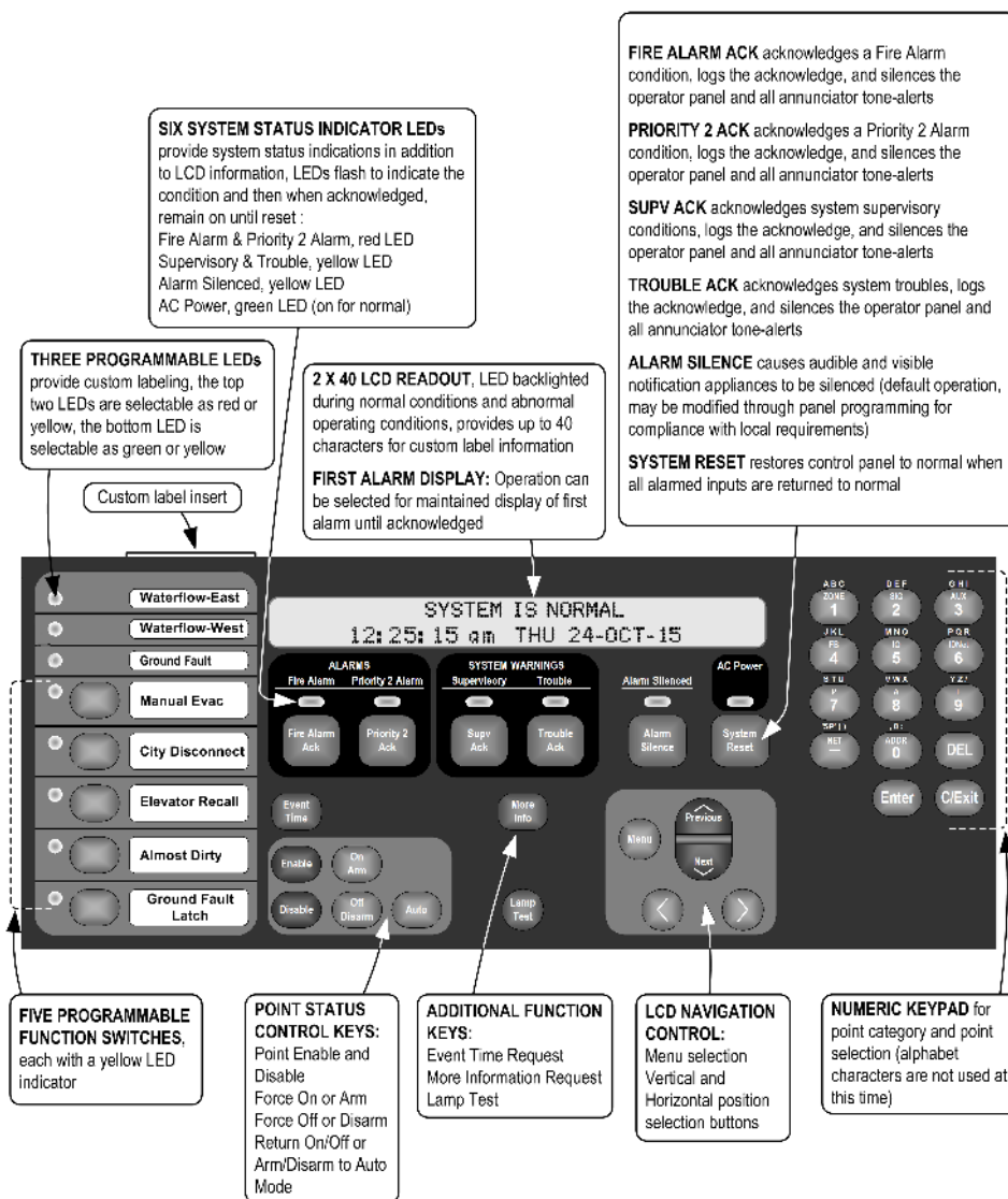
Figure 5: Operator Interface
